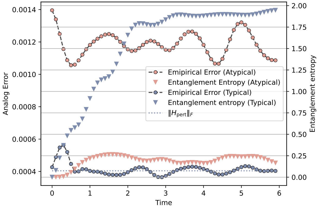
QIMF, one segment evolution with disorder & imperfections
